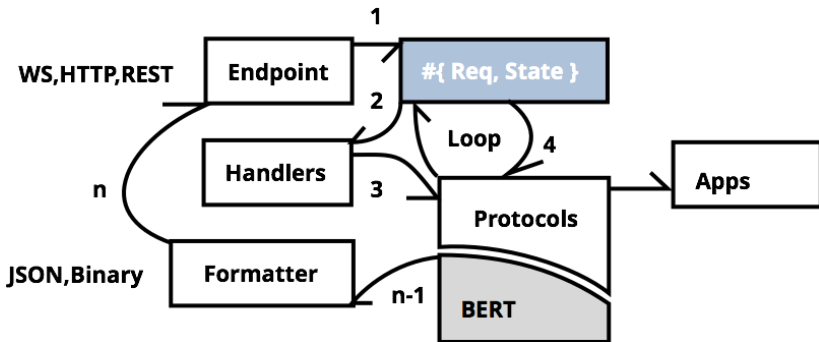
Figure 4: Messaging Pipeline
